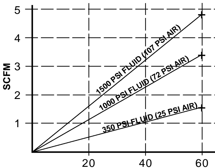
Pump Air Consumption
